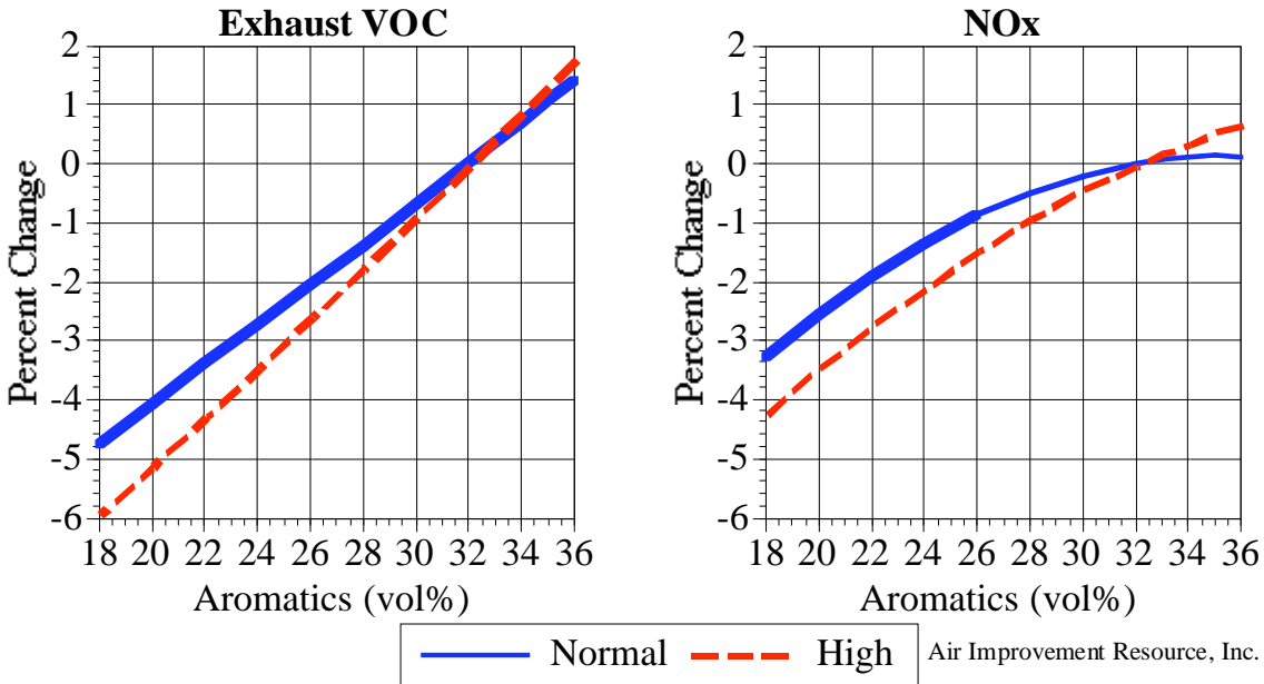
Emission Percent Change vs Aromatics and Emitter Class EPA Complex Model
