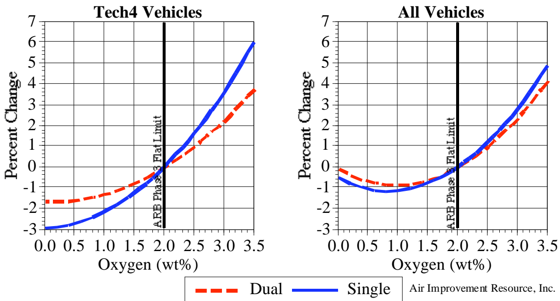
NOx Emissions Percent Change from Reference Fuel vs Oxygen ARB Draft3 Predictive Model
